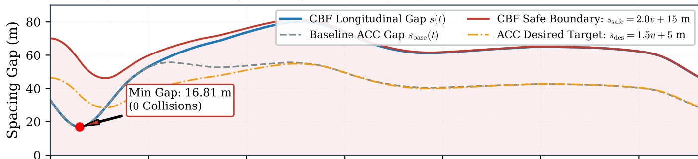
(a) Longitudinal Following Spacing & Headway Expansion
