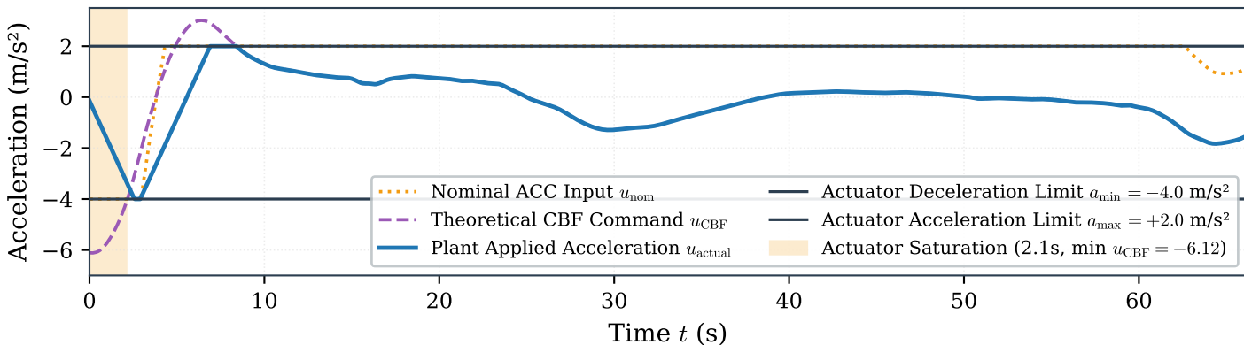
(c) Control Intervention, Braking Saturation, and Rate-Limiting
