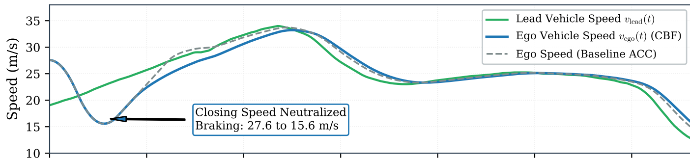
(c) Control Intervention, Braking Saturation, and Rate-Limiting
